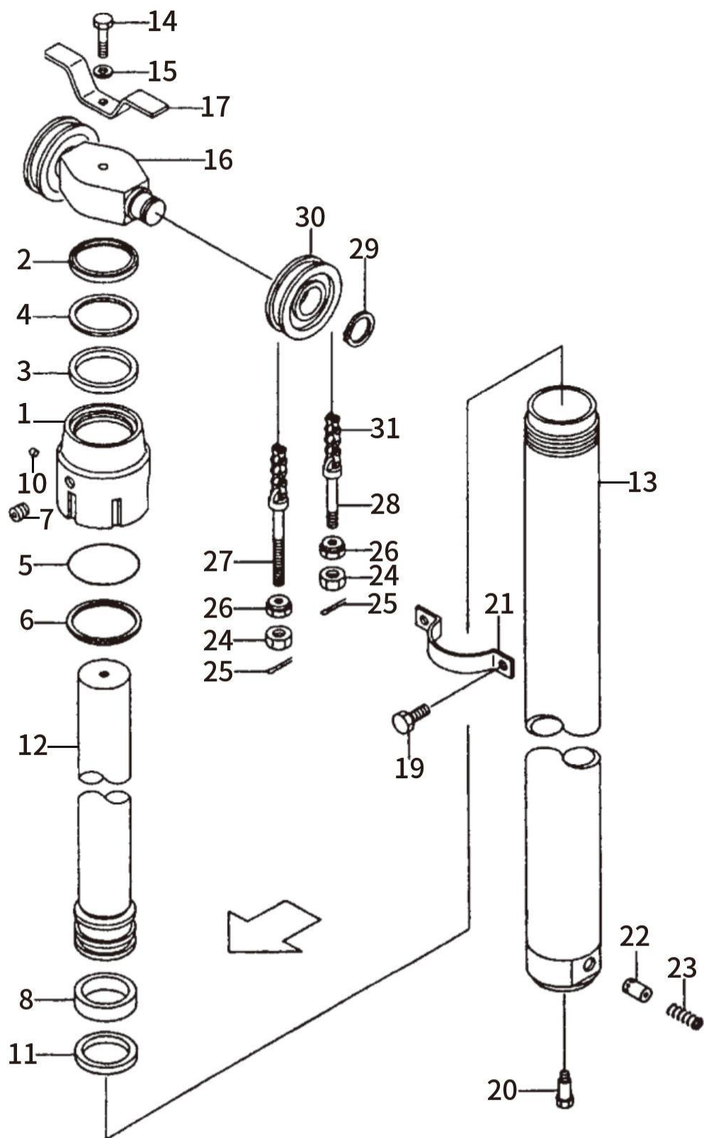
FIG.50-2 LIFT CYLINDER(FRONT) [VFM11E] [VFHM11E] 图 50-2
