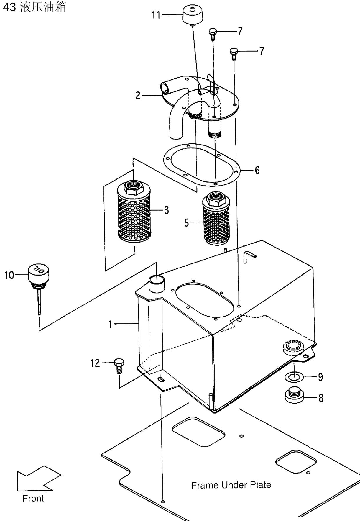
FIG.43 OIL TANK
