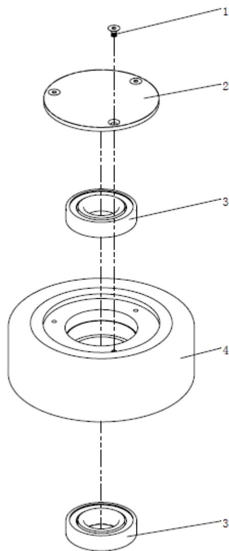
1.6 The front wheel parts
